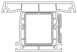
14x345 with 249035 and 259023
