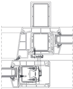
aluplast smart-slide with static post 209294, 249035, 259926
