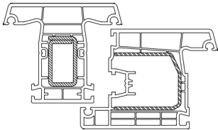
14x328 with 209193 14x341 with 229098
