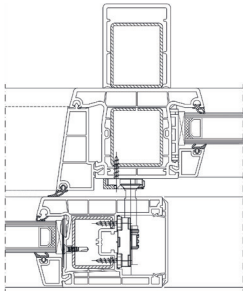
aluplast smart-slide with static post 209294, 249035, 229125
