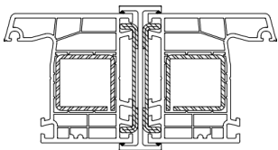
2 x 14x307 with 259106 14x267 with 2x 209900
