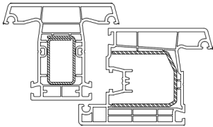
14x328 with 209193 14x341 with 229101
