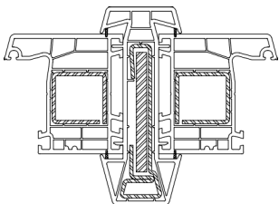
2 x 14x307 with 259106 14x218 with 289218 and 70mm x 6mm flat bar
